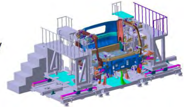
CKD assembly
