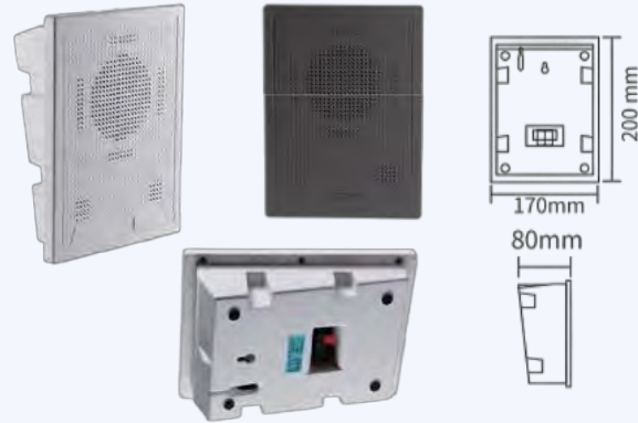
Wall mounted speaker KD-705 (Surface mounted/recessed) (B&W)
